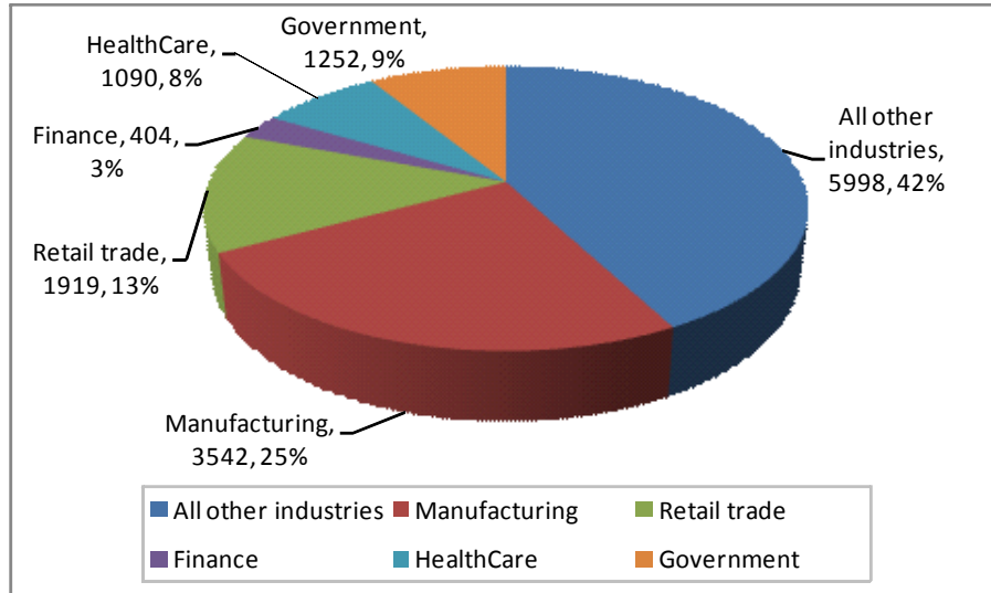
Graph1 Employment by Industry in Montgomery County
